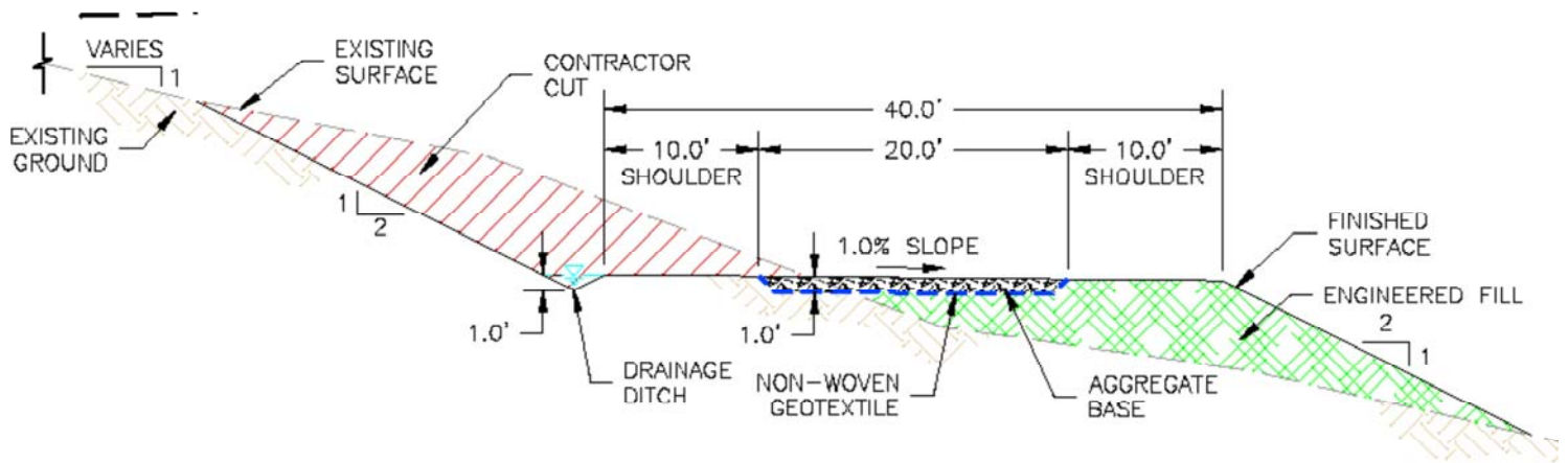
CRANE ACCESS ROAD SECTION (TYPICAL) NOT TO SCALE
